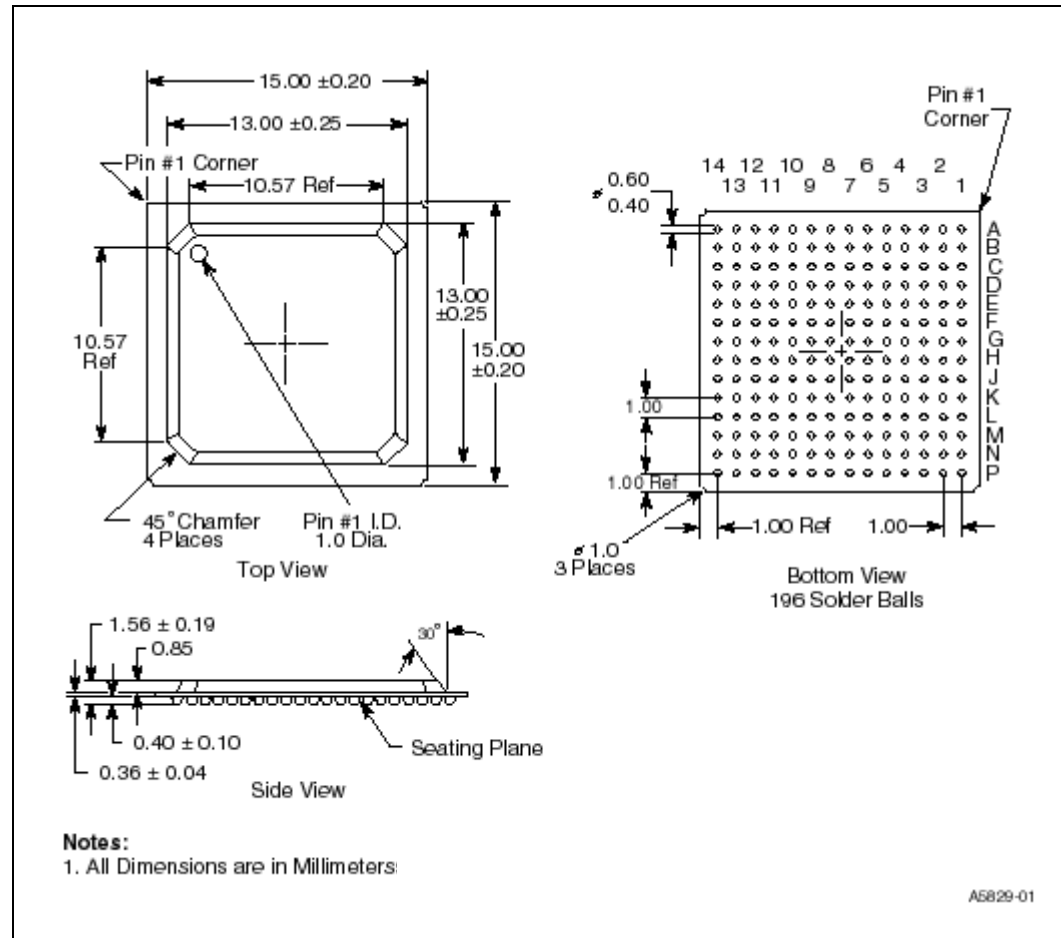
Figure 34. Dimension Diagram for the 82559ER 196-Pin BGA
