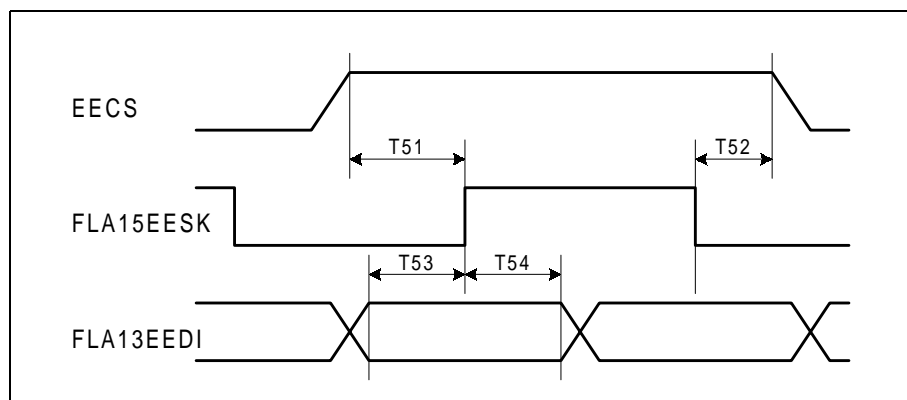
Figure 31. EEPROM Timings
